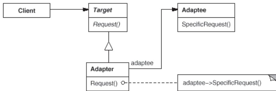
Figure 6: The structure of the Adapter pattern, the object approach.
