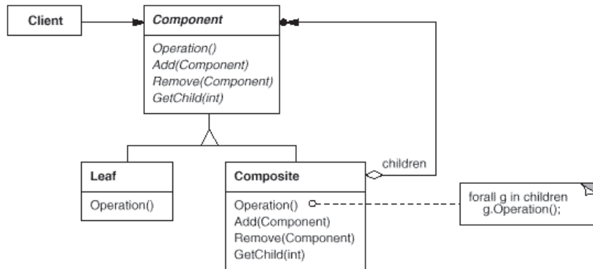
Figure 8: The structure of the Composite pattern.
