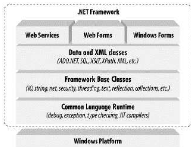
Figure 2: The .NET Framework.
